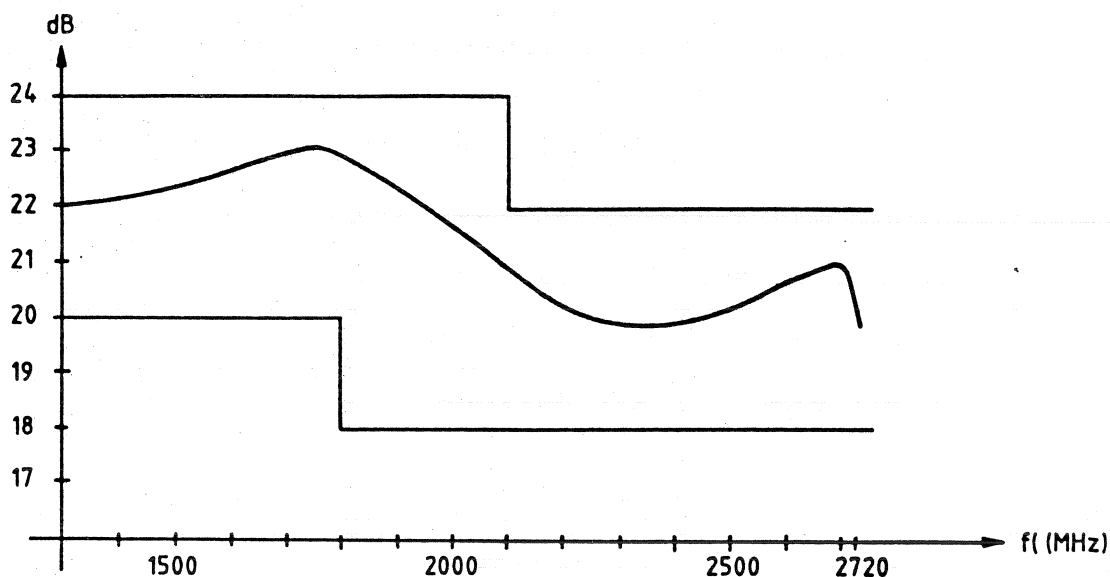
Fig. 5-1 Typical frequency response curve with tolerance limits
